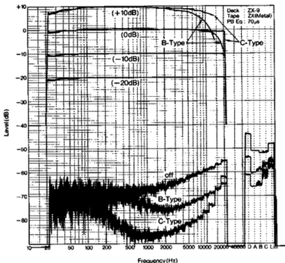
Frequency Response and Noise Spectrum Analysis
