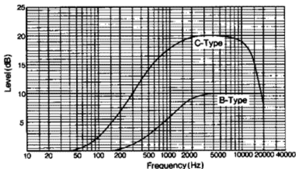
Low-level Encoding Characteristics (-60 dB)
